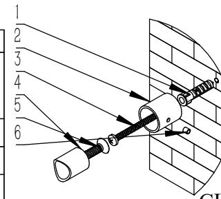
ALLEN KEY 1PCS SMALL SCREW 4PCS WALL PLUG 4PCS SCREW 4PCS
